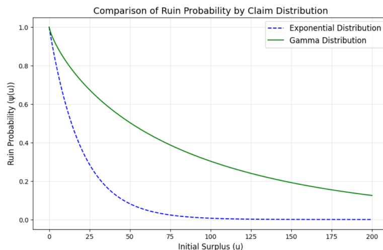
Figure 1. comparison of ruin probability curves based on claims distribution.
